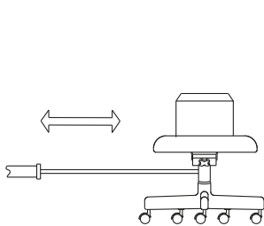
Caster/Chair Base Durability Test: 2,000 cycles over obstruction 98,000 over smooth along a 30" distance with a 250 lb. load.
