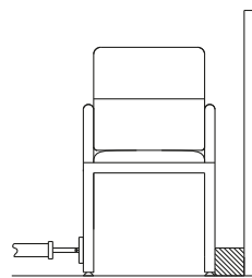
Leg Strength Test - Side Application: 75 lb. force applied, 113 lb. proof load.
