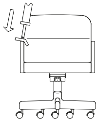
Arm Durability Test: Apply 90 lb. force at 10 degree angle for 60,000 cycles.
