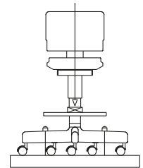
Footrest Durability Test: 100 lb. weight applied along a 4" length of the footrest for 1 minute.
