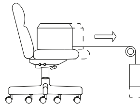
Out Stop Test for Chairs with Manually Adjustable Seat Depth: 163 lb. forward force with 55 lb. downward force for 25 cycles.
