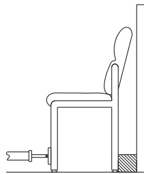
Leg Strength Test - Front Application: 75 lb. force applied, 113 lb. proof load.
